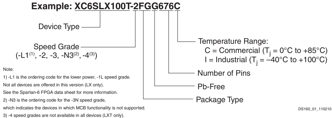
Figure 1: Spartan-6 FPGA Ordering Information
