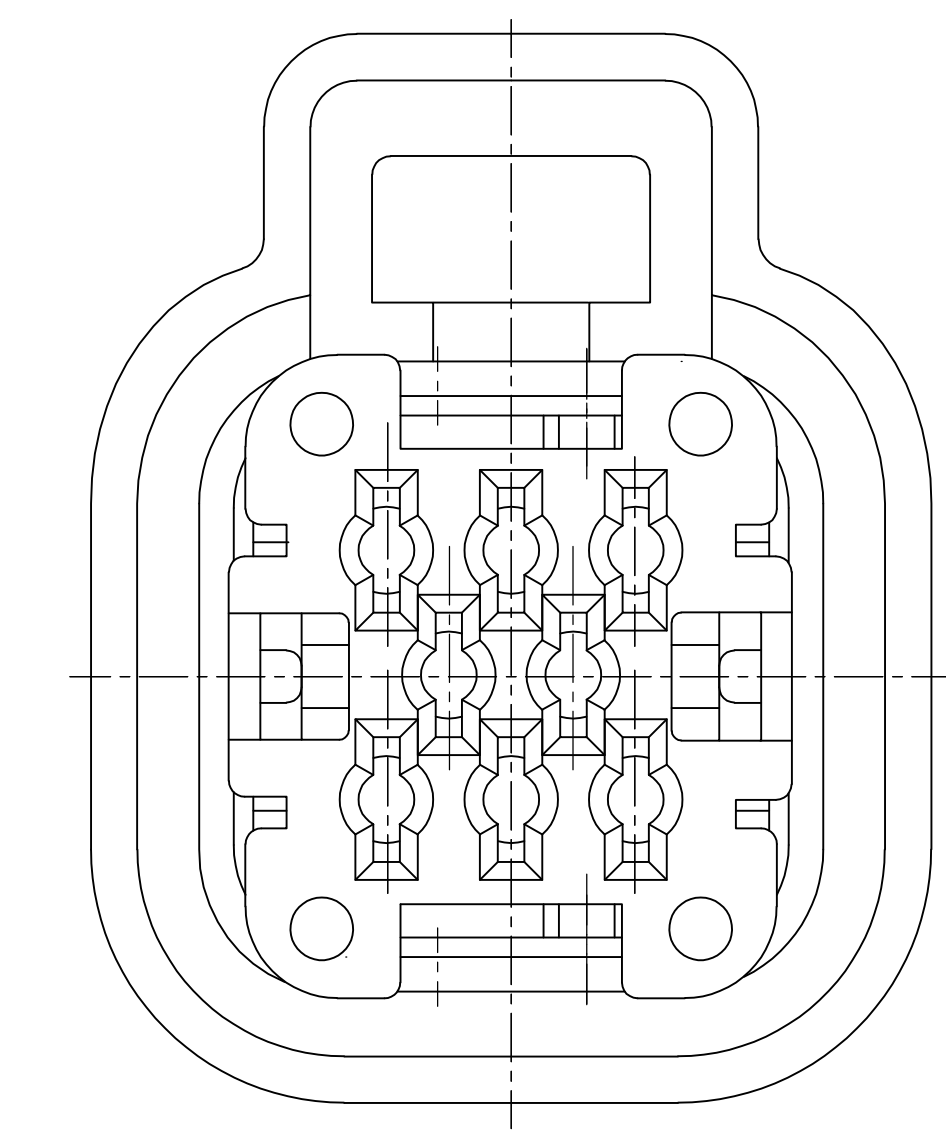
BOTTOM VIEW WITH LOCKING WEDGE
