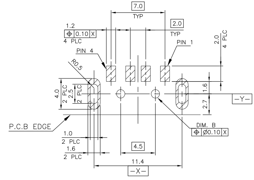
RECOMMENDED PCB LAYOUT (THICKNESS: 1.6mm) (COMPONENT VIEW) TOLERANCE: 1PLC:±0.1 2PLC:±0.05
