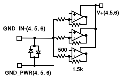
CIRCUIT 5
