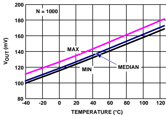
FIGURE 32. EL8173 V_{OUT} LOW vs TEMPERATURE, R_L = 1k , V_+ , V_- = \pm 2.5V
