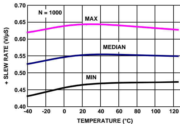
FIGURE 34. EL8173 + SLEW RATE vs TEMPERATURE, INPUT \pm 0.015V @ GAIN + 100
