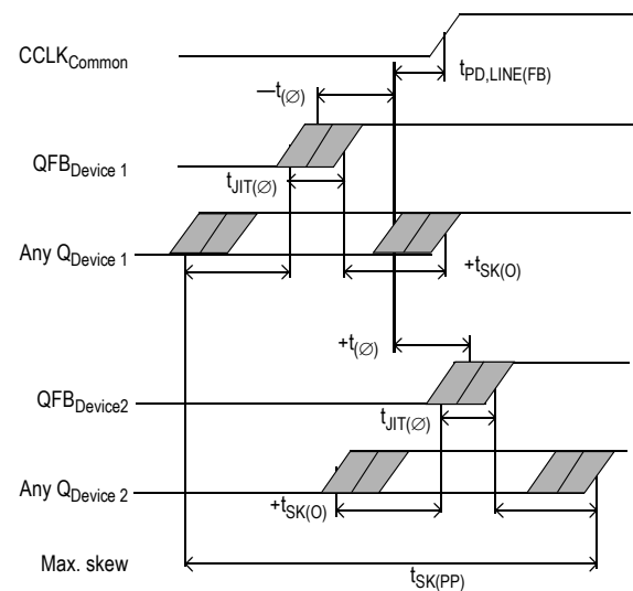
Figure 8. MPC93R52 Max. Device-to-Device Skew
