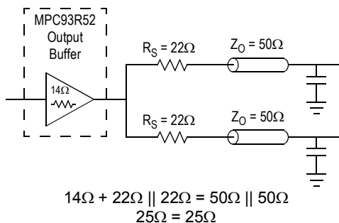
Figure 12. Optimized Dual Line Termination
