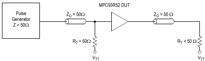
Figure 13. CCLK MPC93R52 AC Test Reference for V_{CC} = 3.3 V and V_{CC} = 2.5 V
