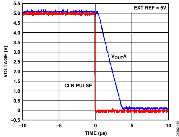
Figure 50. Hardware \overline{\text{CLR}}
