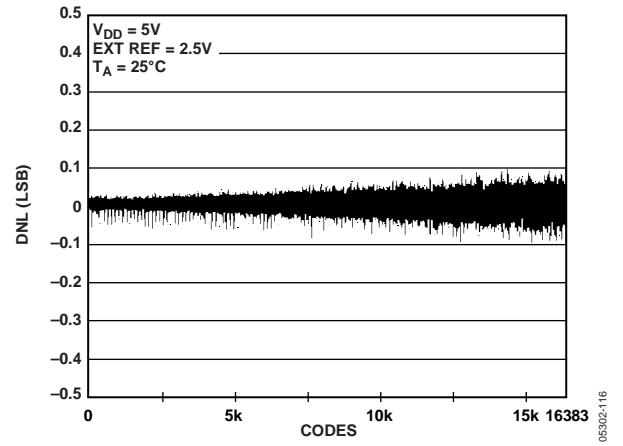
Figure 16. DNL AD5648-2
