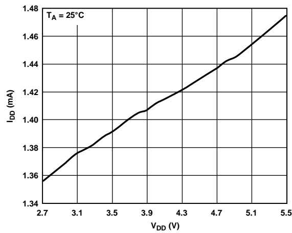
Figure 35. Supply Current vs. Supply Voltage
