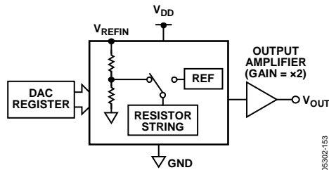
Figure 53. DAC Architecture
