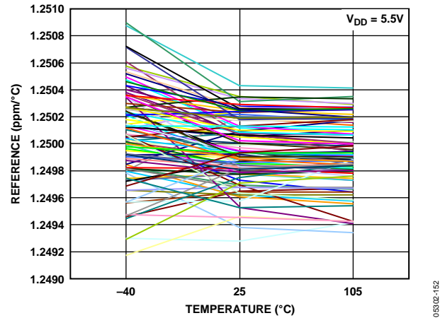
Figure 52. 1.25 V Reference Temperature Coefficient vs. Temperature
