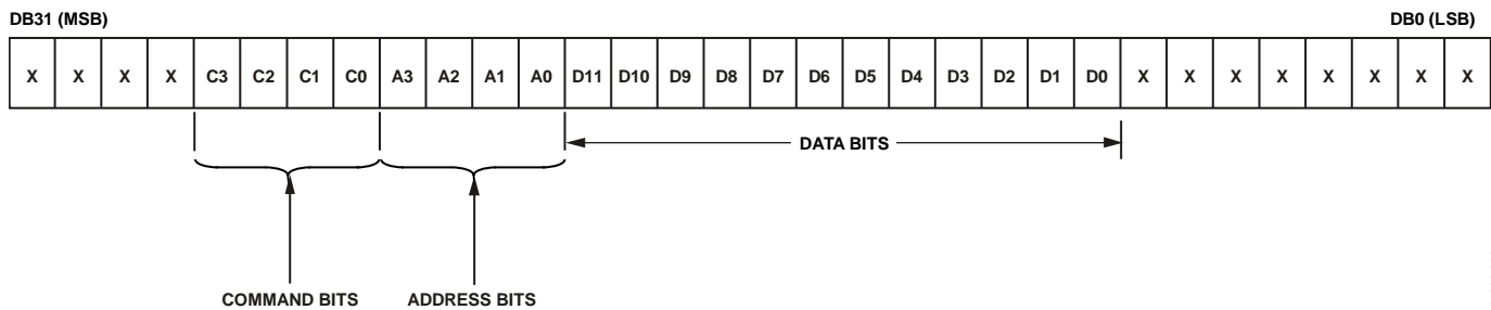
Figure 57. AD5628 Input Register Contents
