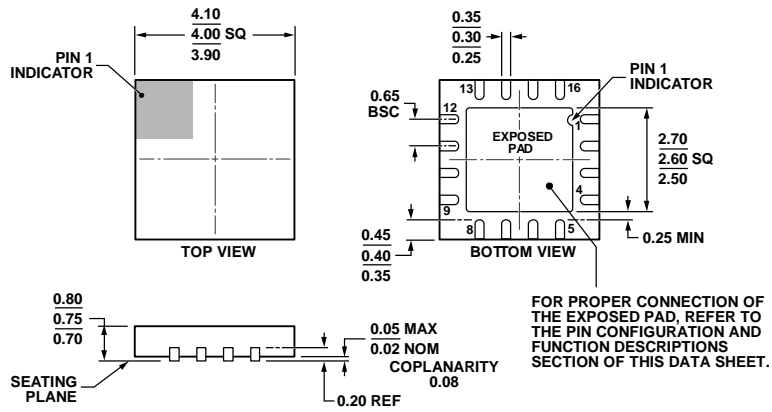
Figure 62. 16-Lead Lead Frame Chip Scale Package [LFCS-P-WQ] 4 mm × 4 mm Body, Very Very Thin Quad (CP-16-17)
