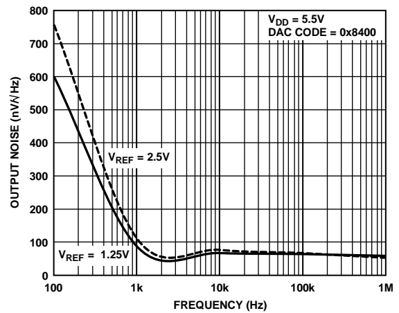
Figure 47. Noise Spectral Density, Internal Reference
