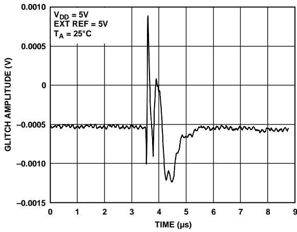
Figure 42. Analog Crosstalk
