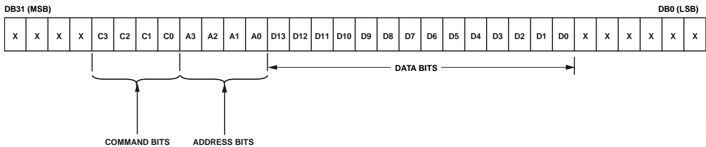
Figure 56. AD5648 Input Register Contents
