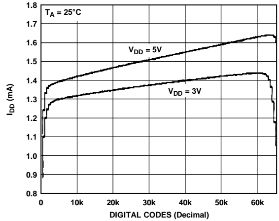
Figure 33. Supply Current vs. Code
