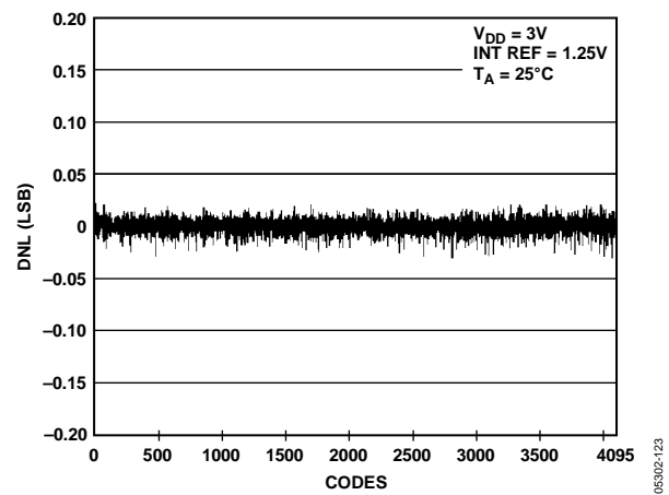
Figure 23. DNL AD5628-1
