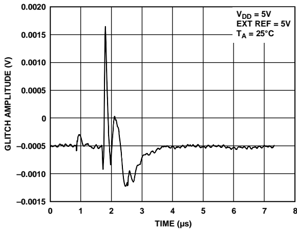
Figure 43. DAC-to-DAC Crosstalk
