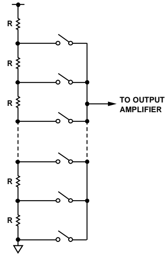
Figure 54. Resistor String
