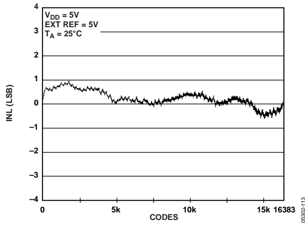
Figure 13. INL AD5648-2
