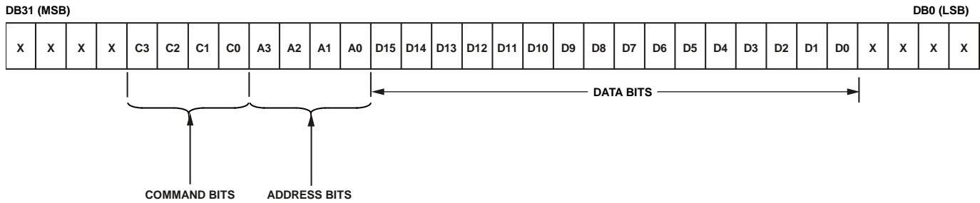
Figure 55. AD5668 Input Register Contents
