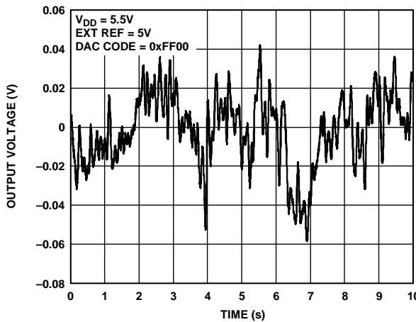
Figure 44. 0.1 Hz to 10 Hz Output Noise Plot, External Reference
