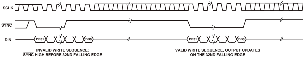
Figure 58. \overline{\text{SYNC}} Interrupt Facility
