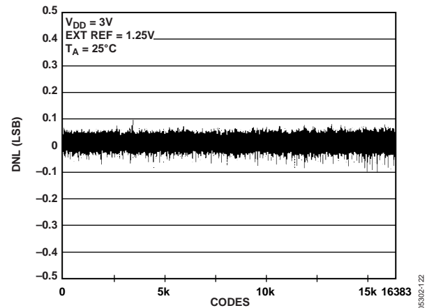
Figure 22. DNL AD5648-1
