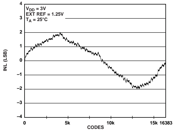
Figure 19. INL AD5648-1
