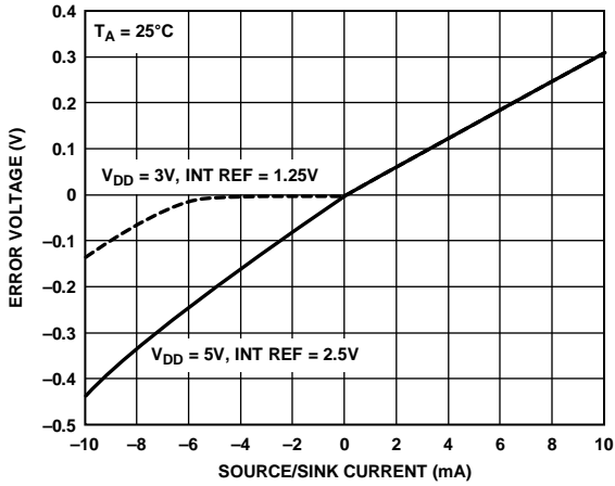
Figure 30. Headroom at Rails vs. Source and Sink
